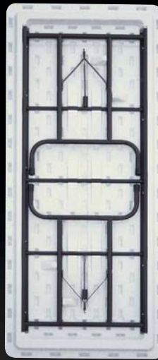
Strong steel frame, with five tubular supports
